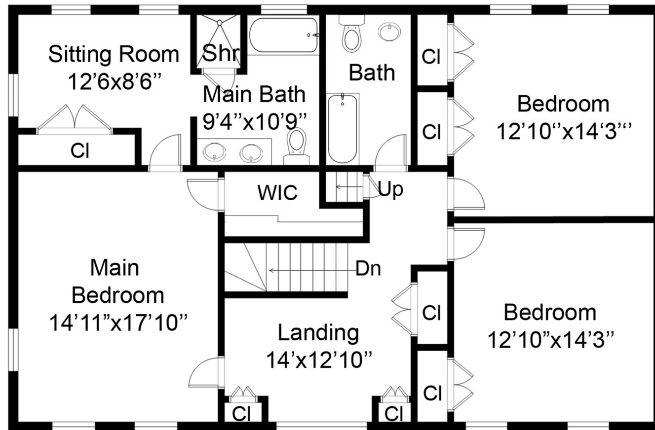
SECOND FLOOR - SOUTH WING
