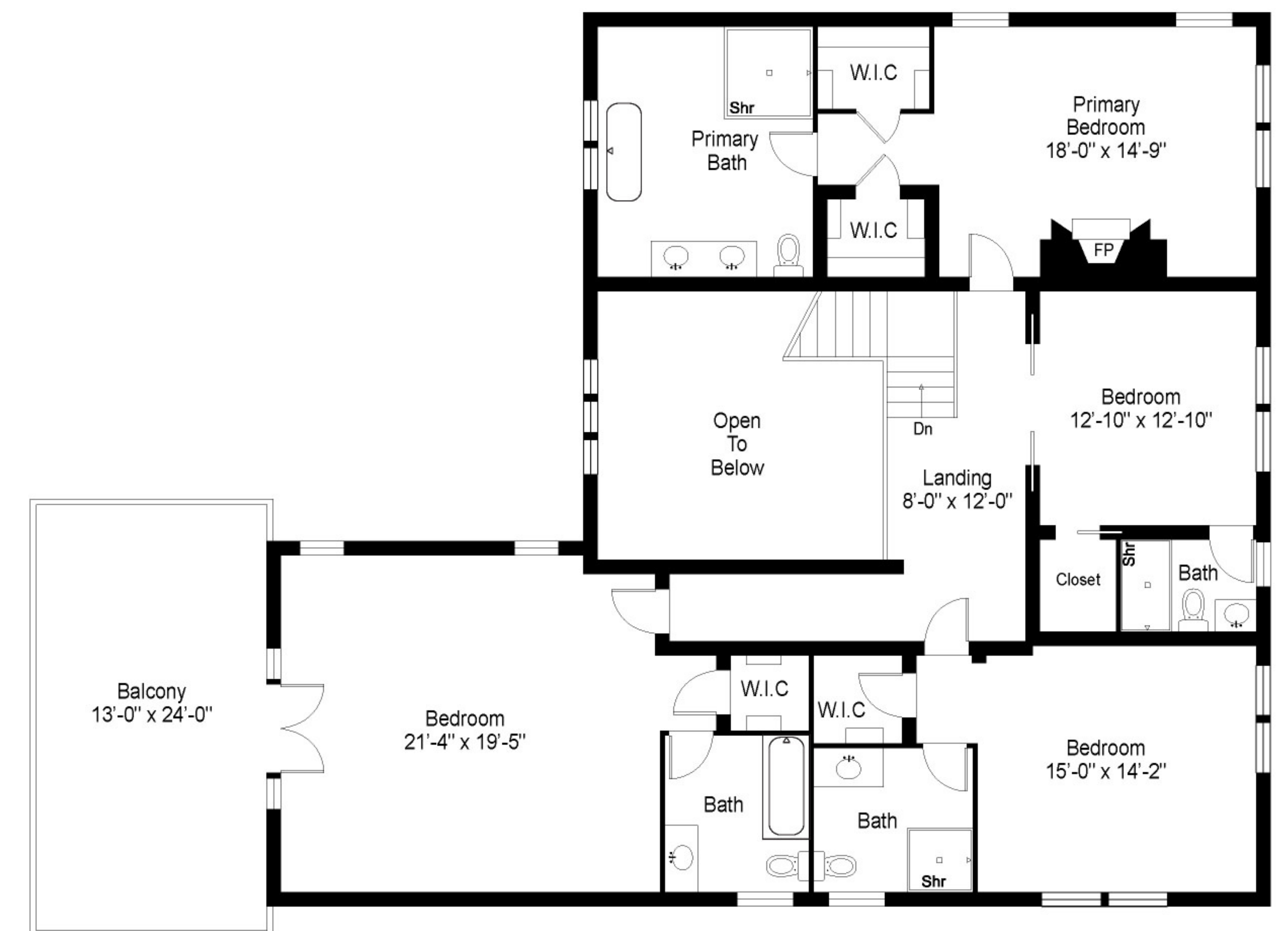
SECOND FLOOR
