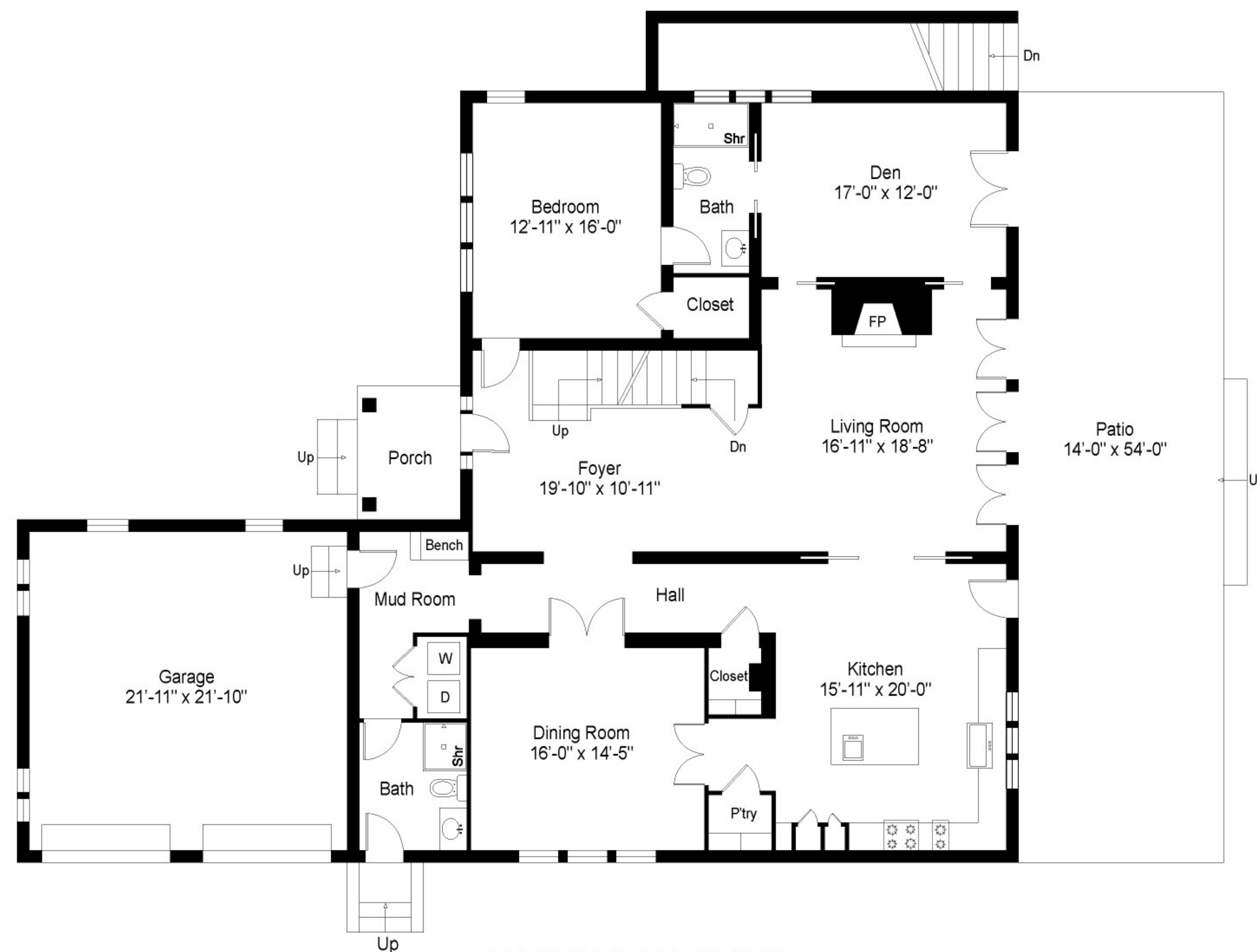
FIRST FLOOR
