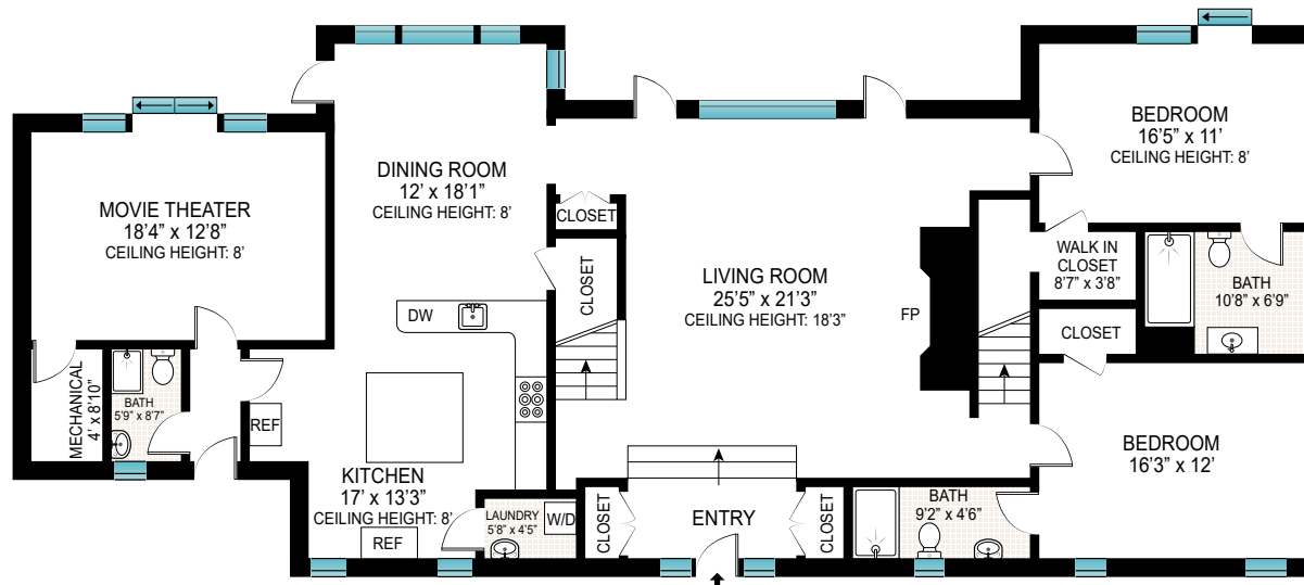
FIRST FLOOR CEILING HEIGHT: 8'
