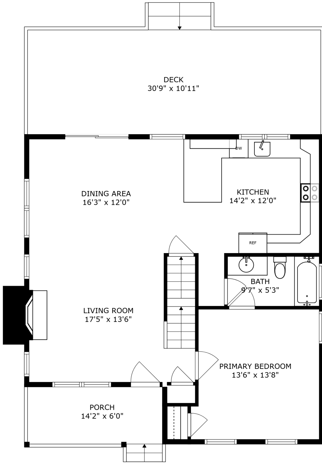
FLOOR 2
