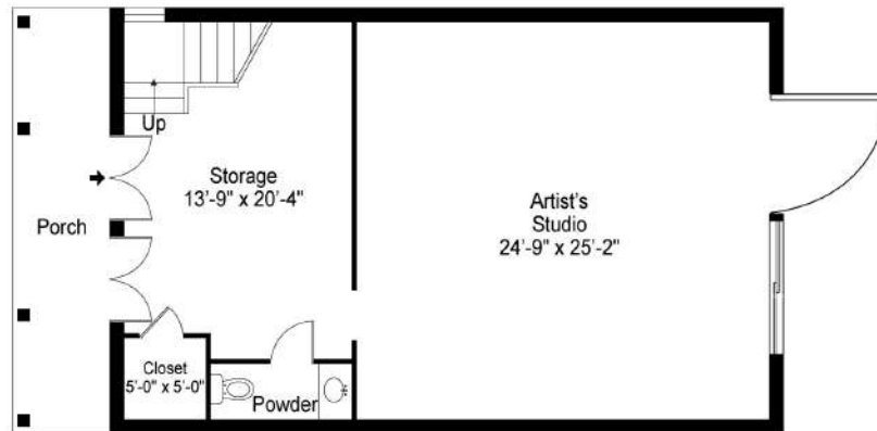
STUDIO FIRST FLOOR
