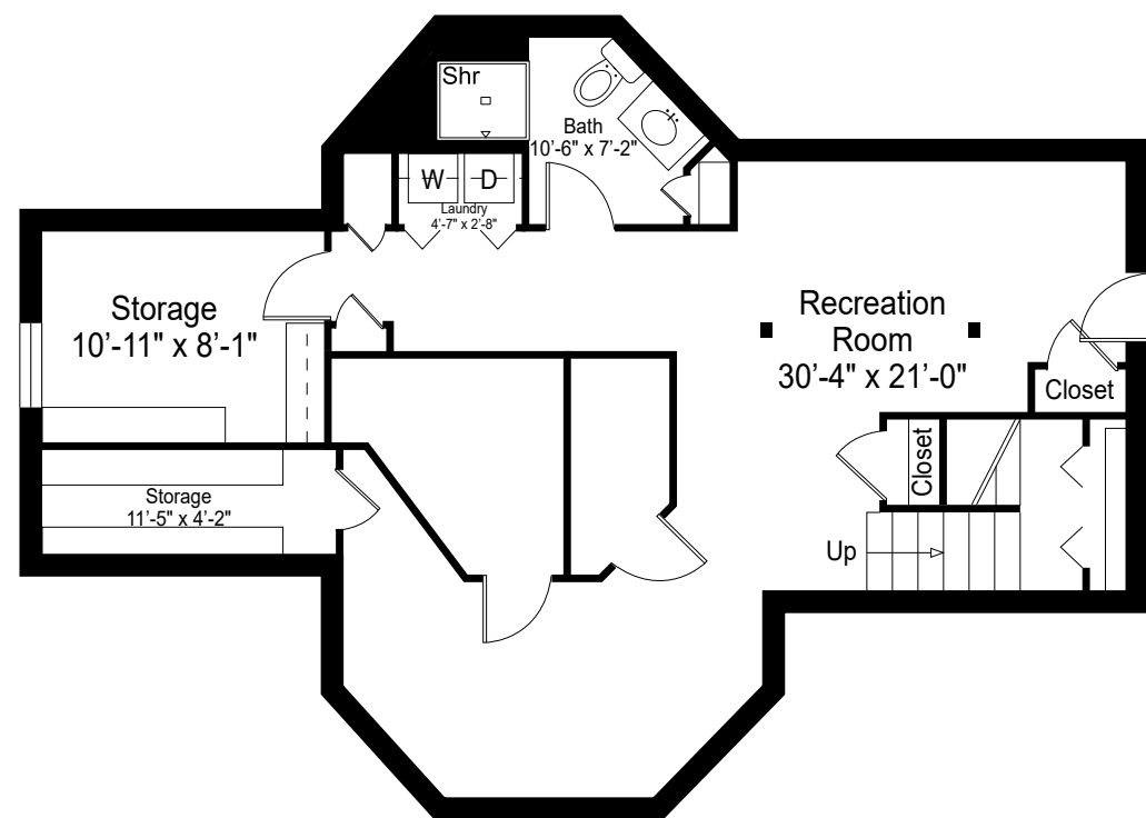
FLOOR 1
