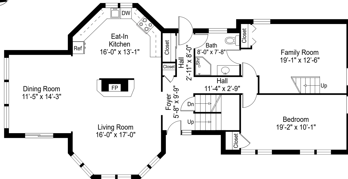
FLOOR 2
