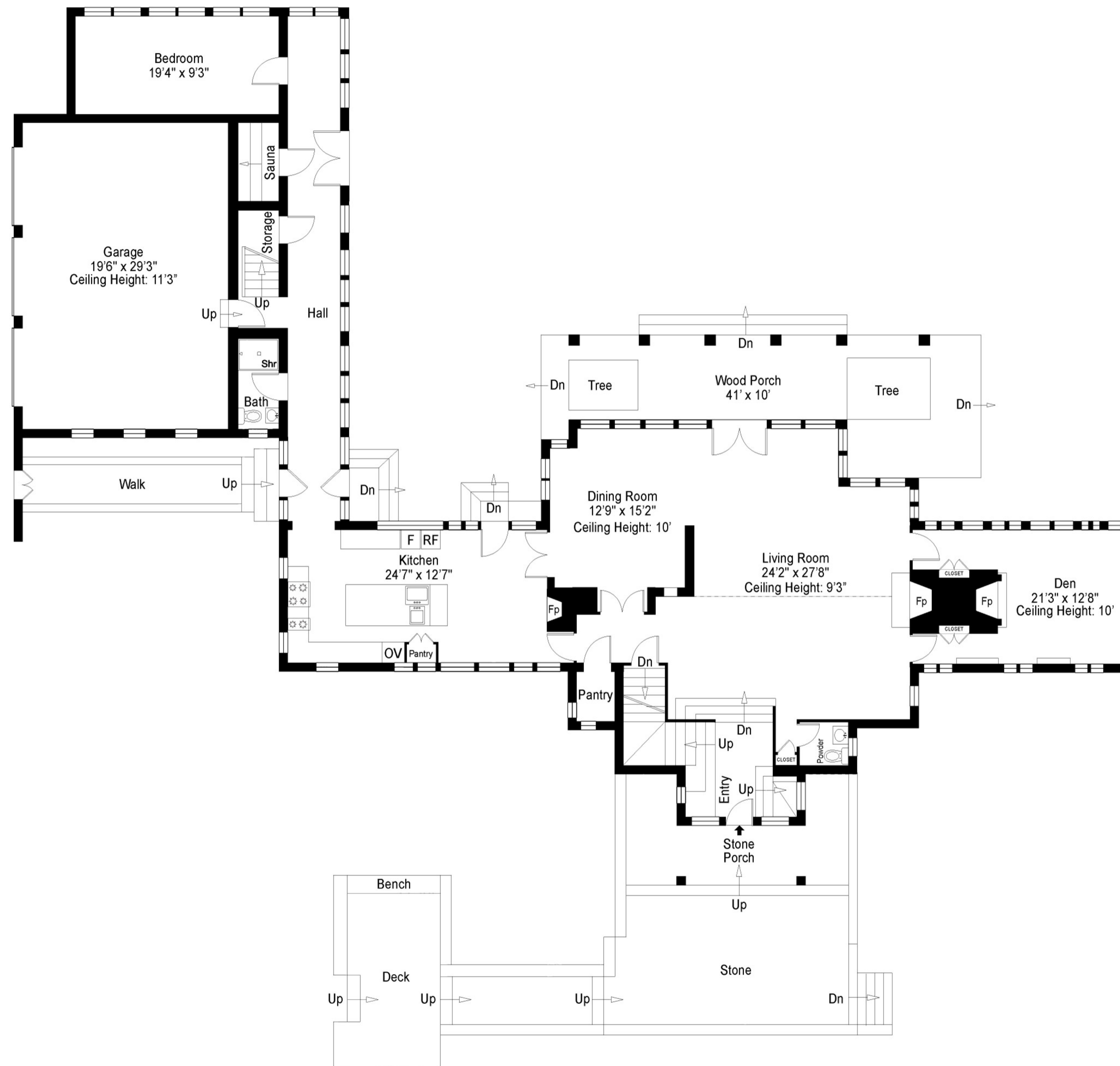
FIRST FLOOR
