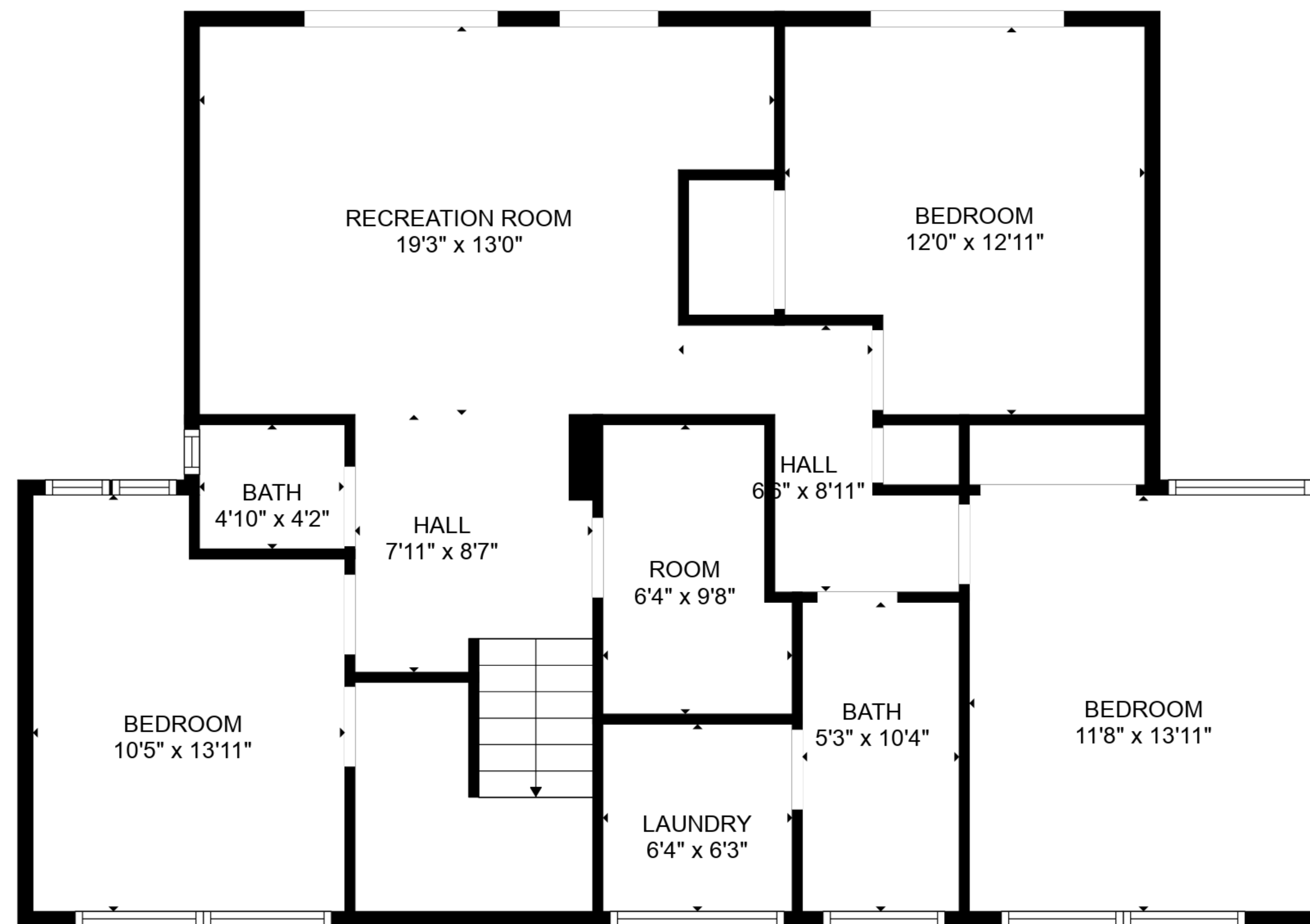
FLOOR 2
