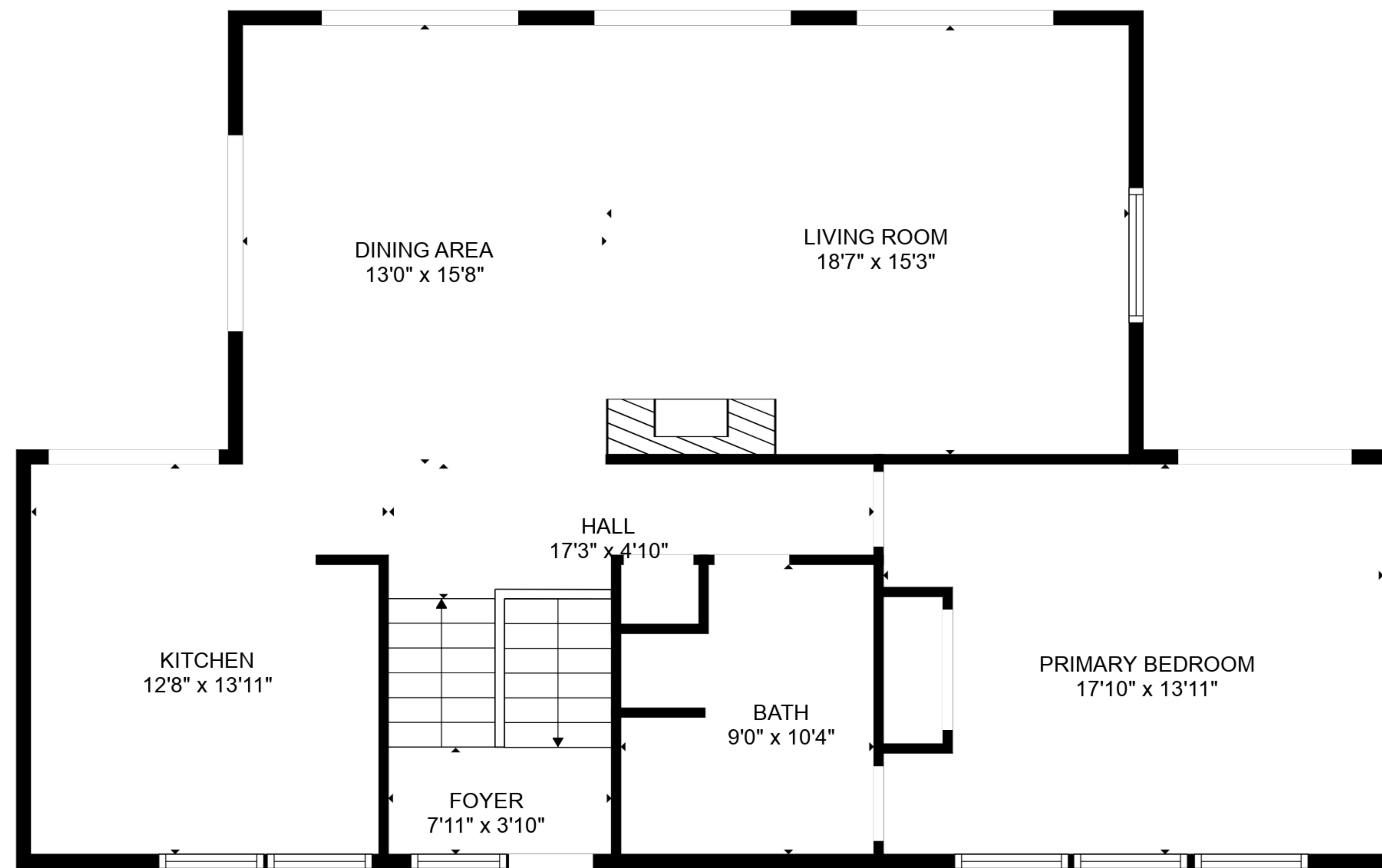
FLOOR 2
